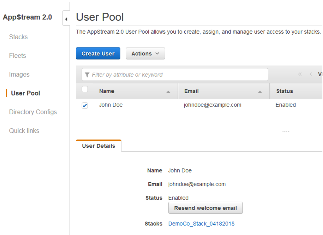
Figure 11: The User Pool dashboard showing the newly created user with a stack now assigned.
