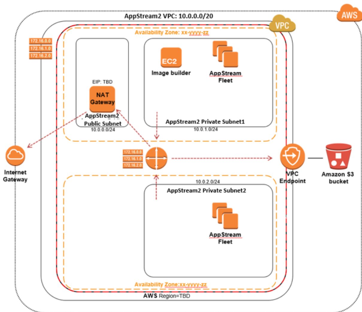
Figure 15: DemoCo VPC architecture.
